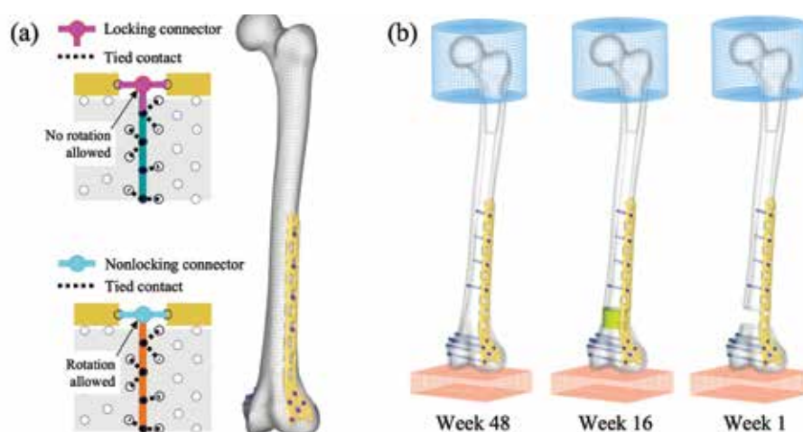
Figure 3. (a) Schematic of locking and nonlocking connectors in femur-plate-screw FE model. (b) Week 48, Week 16, and Week 1 FE models with axial loading boundary conditions (transparency applied for screw visualization).
